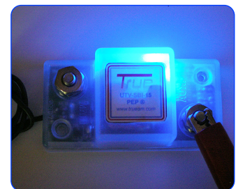
UTV-SBI-15 with insulators 12" Black Cable w/Lugs 12" & 18" Red Cables w/Lugs 3M Dual Lock® fastener
